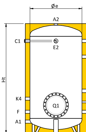
Couplings chart
