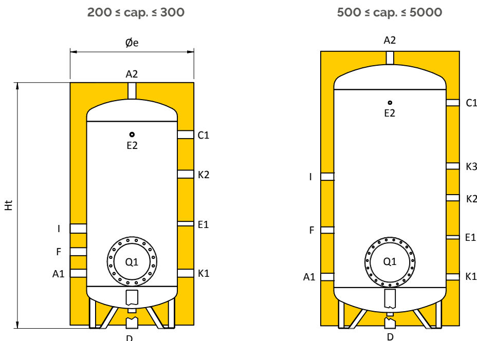
Couplings chart
