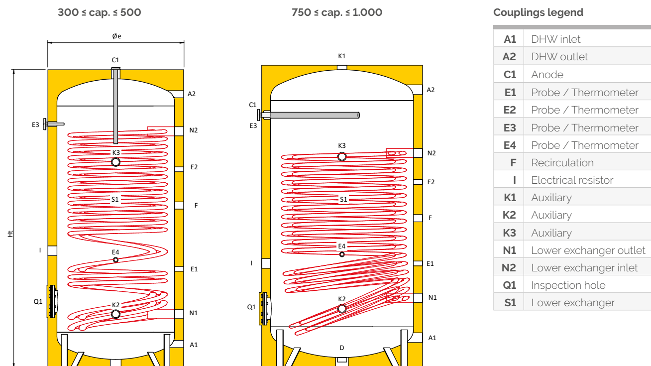
Couplings chart
