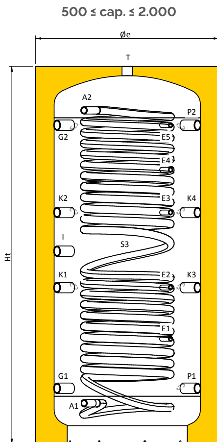
Couplings chart
