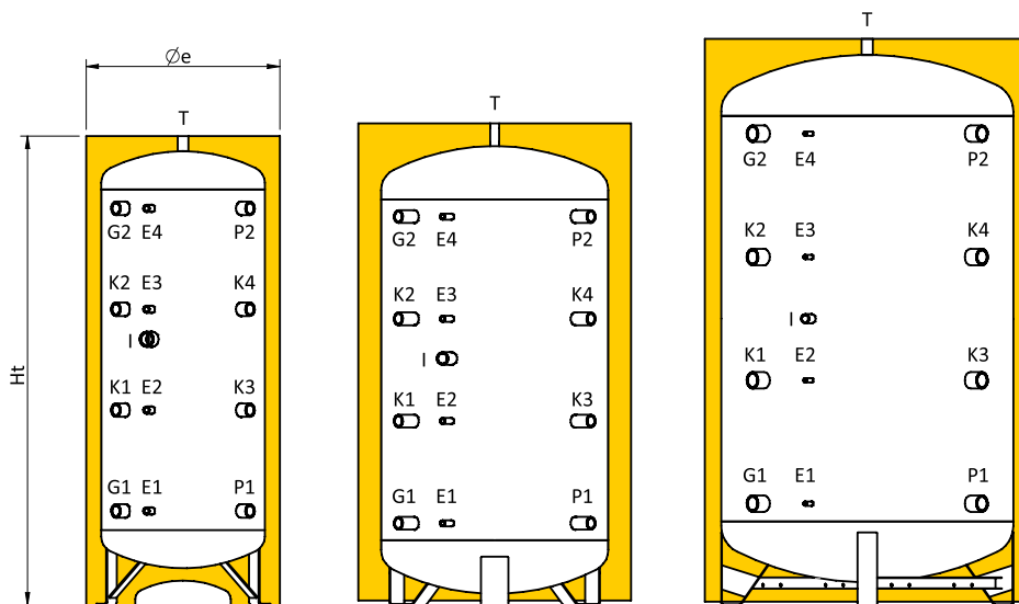
Couplings chart
