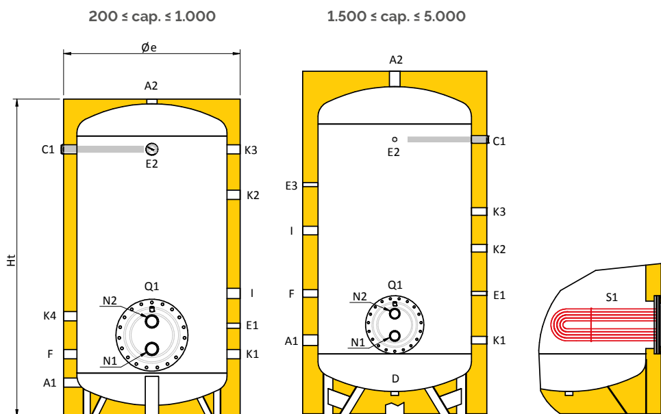
Couplings legend
