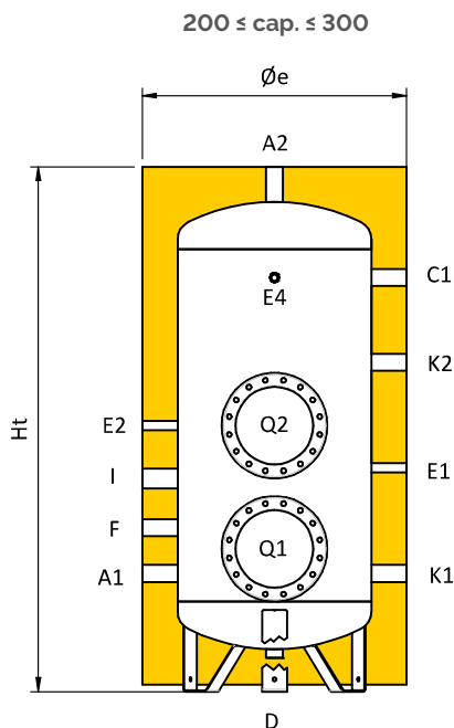
Couplings chart
