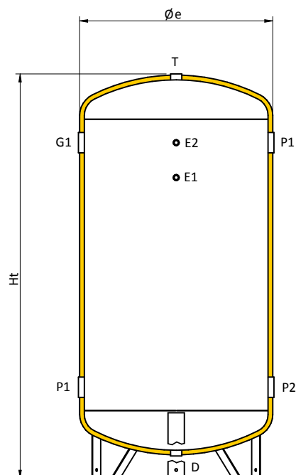
Couplings chart
