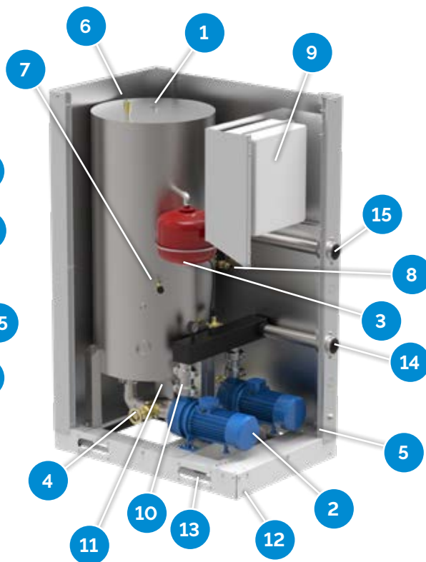
Vertical HPT
