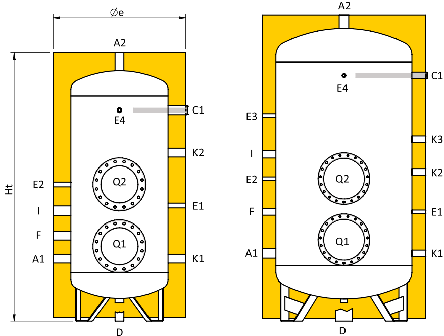
Couplings chart
