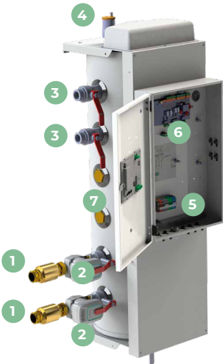
HRC 70 cascade installation from 40 to 96 kW
