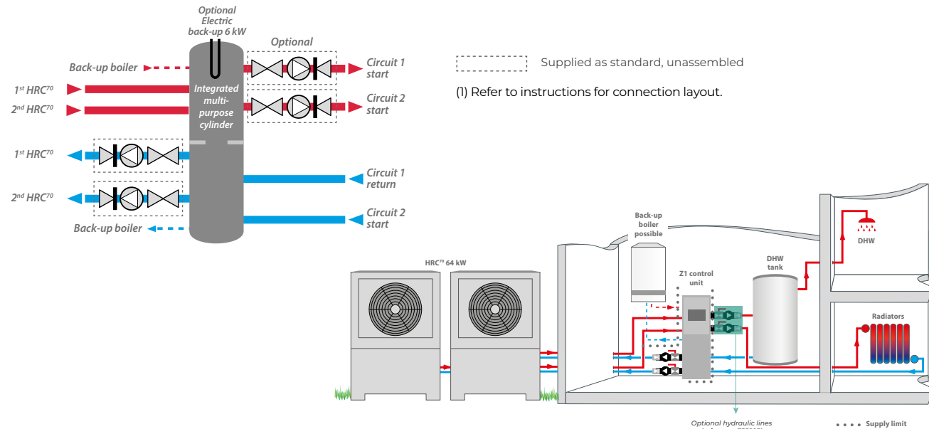
Schematic diagram CASCADE (1) : HRC 70 Z1 control unit
