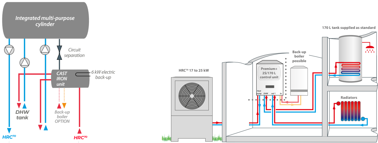
Schematic diagram (1) : HRC 70 - premium+ 2S/170 L
