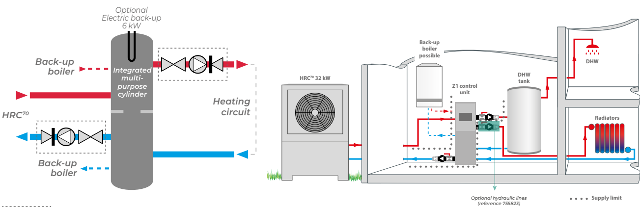
Schematic diagram (1) : HRC 70 Z1 control unit
